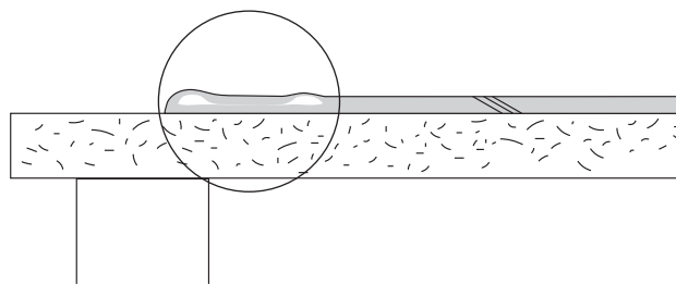
Figure 8: Cutaway showing Bubbles caused by faster fusing of the edges and consequent air entrapment between layers.
